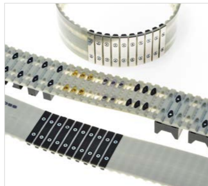
BRECO® ATN-System
